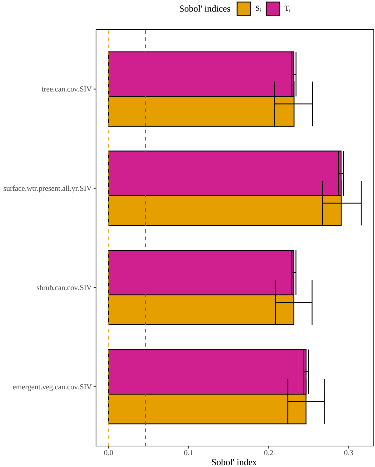
Figure 4. Results of a sensitivity analysis for the minkPaluForestedOrShrubMore405ha model based on an arithmetic mean structure. Dashed lines represent baseline numerical approximation error for S_i and T_i ( i.e. , dummy variables).
